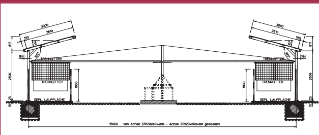
Cross section of horse walker with partial roof
