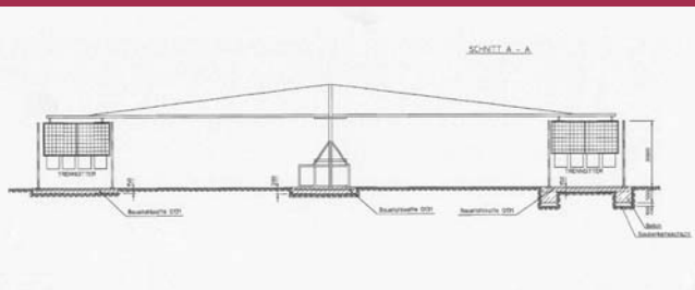
Cross section of horse walker with panel fence
